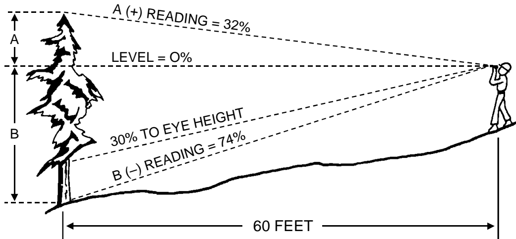
Measuring tree height on sloping ground using a percent clinometer and a baseline distance other than 100 feet.
