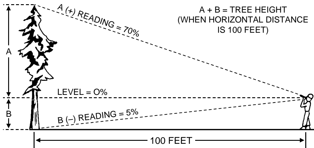
Measuring tree height on flat ground using a percent clinometer and a 100-foot baseline distance.
