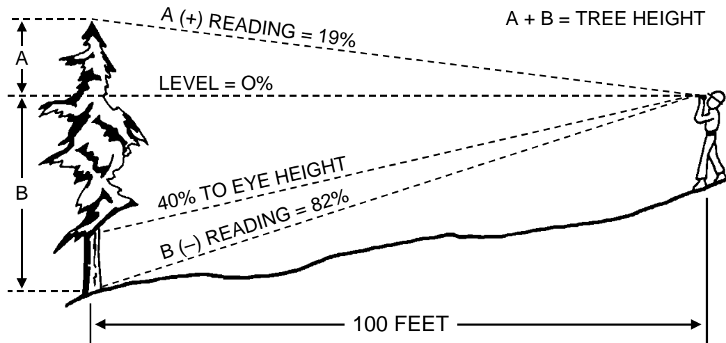
Measuring tree height on sloping ground using a percent clinometer and a 100-foot baseline distance.
